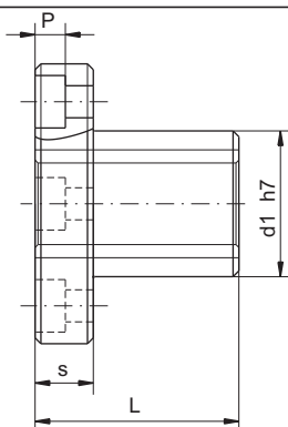
Od Tr 10 x 3 do Tr 22 x 5 4 luknje From Tr 10 x 3 to Tr 22 x 5 4 holes
