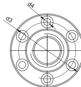
Od Tr 24 x 5 do Tr 60 x 9 6 lukenj From Tr 24 x 5 to Tr 60 x 9 6 holes
