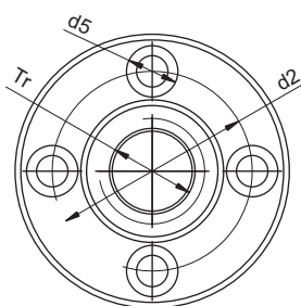
Od Tr 10 x 3 do Tr 22 x 5 4 luknje From Tr 10 x 3 to Tr 22 x 5 4 holes
